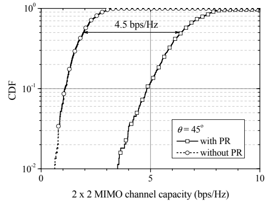
Figure 9 The CDF of the 2 \times 2 MIMO channel capacity with/without 4-unit PR for \theta = 45^\circ (received noise level=-90 dBm/Hz).
