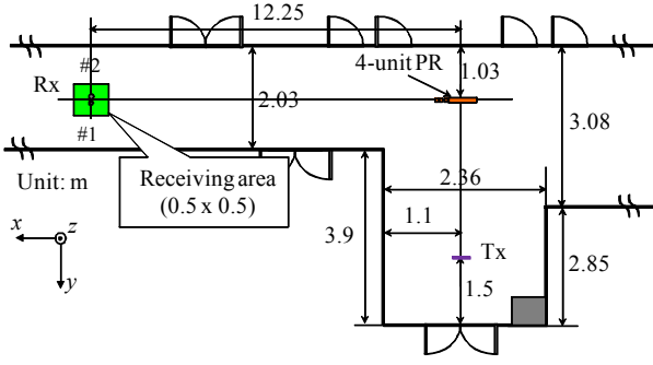
Figure 3 MIMO measurement environment.
