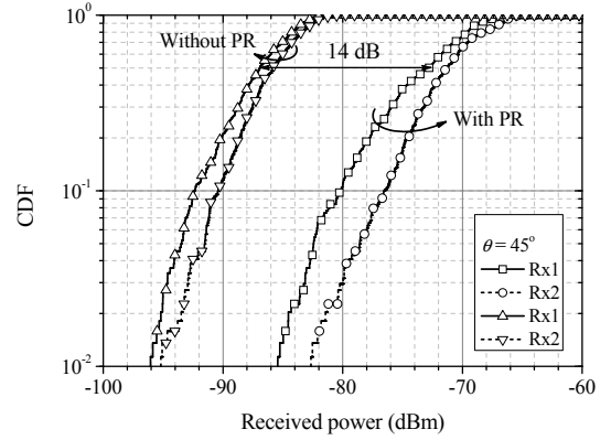
Figure 5 The CDF of the received power with/without 4-unit PR for \theta = 45^\circ (received noise level=-120 dBm/Hz).
