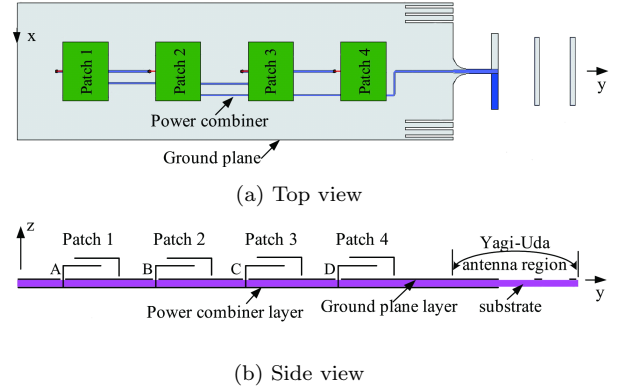
Figure 1 Configuration of one-unit PR.
