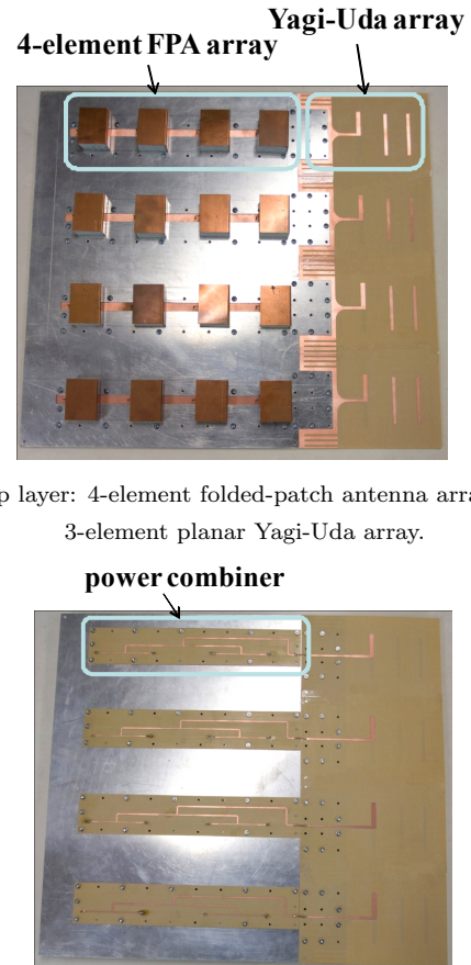
(a) Top layer: 4-element folded-patch antenna array and a 3-element planar Yagi-Uda array. (b) Bottom layer: Microstrip power combiner. Figure 2 Photographs of the fabricated 4-unit PR.
