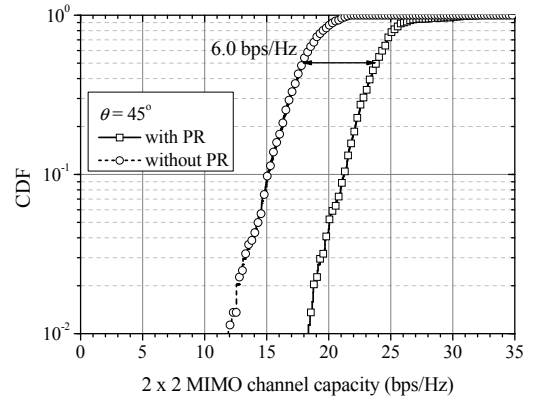
Figure 6 The CDF of the 2 \times 2 MIMO channel capacity with/without 4-unit PR for \theta = 45^\circ (received noise level=-120 dBm/Hz).
