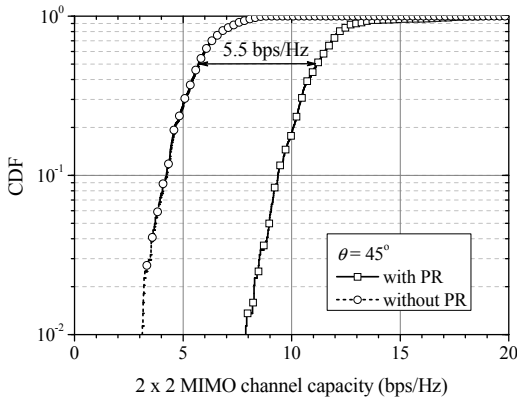
Figure 8 The CDF of the 2 \times 2 MIMO channel capacity with/without 4-unit PR for \theta = 45^\circ (received noise level=-100 dBm/Hz).
