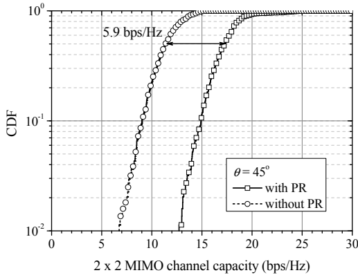
Figure 7 The CDF of the 2 \times 2 MIMO channel capacity with/without 4-unit PR for \theta = 45^\circ (received noise level=-110 dBm/Hz).
