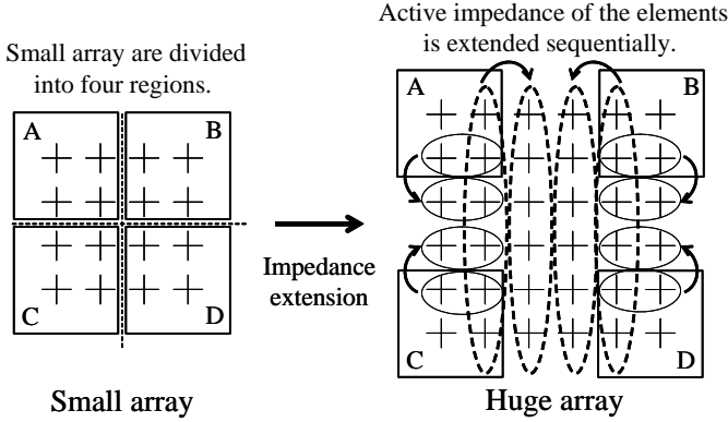
Fig. 2. Two dimensional impedance extension method (IEM).
